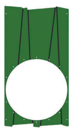
대형입구판넬 D7-2 Large exit board D7-2 T18 X 800 X 1600
