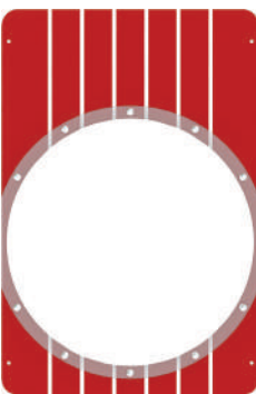
블록판넬 A6 Transparent board A6 T18 X 800 X 1150
