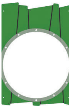
블록판넬 D6 Transparent board D6 T18 X 800 X 1150
