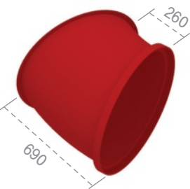
원통 30° Tunnel 30° 690 X 260
