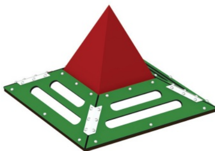
사각뿔지붕C 1240 X 1240 X 860(H) Pyramid roof C
